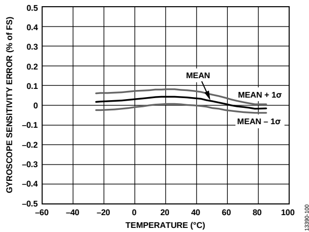
Figure 8. Gyroscope Sensitivity Error vs. Cold to Hot Temperature Sweep
