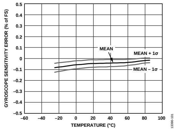
Figure 11. Gyroscope Sensitivity Error vs. Hot to Cold Temperature Sweep
