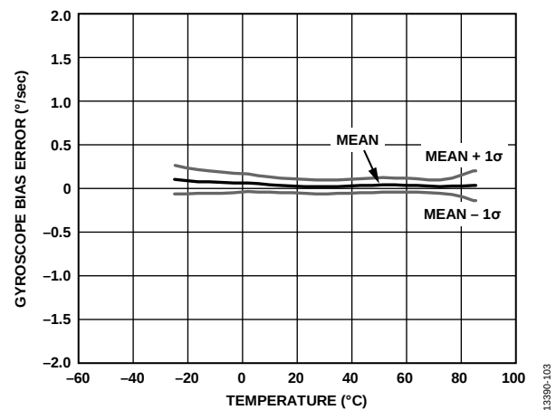
Figure 12. Gyroscope Bias Error vs. Hot to Cold Temperature Sweep
