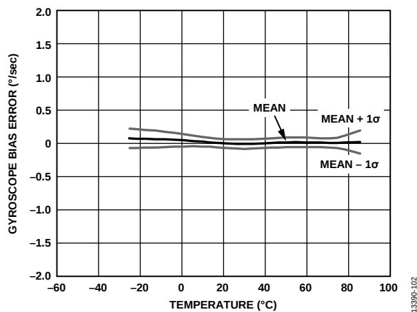
Figure 9. Gyroscope Bias Error vs. Cold to Hot Temperature Sweep
